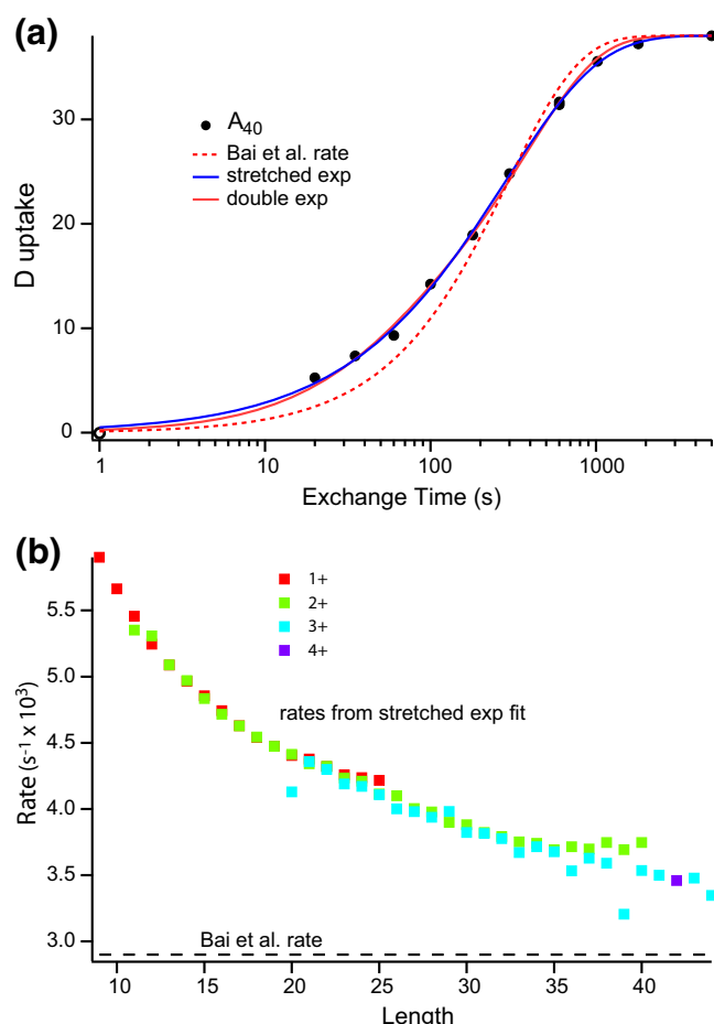
Figure 1. PDLA exchange: (a) deuterium uptake of a 40 residue peptide from random heterogeneously polymerized D,L-alanine. PDLA samples were exposed to H to D exchange (15 °C in 90% D_2O at pD_{read} of 4.01) for increasing times, samples quenched at pH 2.4, 0 °C to essentially halt exchange, and injected into an online system where they were desalted on a small C8 column, and separated by size in a C18 column. The eluant was introduced by electrospray into a Thermo LTQ Orbitrap XL mass spectrometer which further separates peptides by mass and allows time-dependent deuterium uptake of the differently sized PDLA peptides to be measured. Deuterium loss due to back exchange during the analysis was corrected for using an “all D” sample initially fully exchanged in the same buffer. The point shown at 1 s is a zero time control which was injected immediately after simultaneous addition of quench and D_2O buffer. The dashed line shows the single exponential rate predicted from the Bai et al. parameters for large poly peptides. The blue and red solid lines show single stretched exponential and double exponential fits. (b) Stretched exponential rates as a function of PDLA polymer length. The dashed line along the bottom indicates the reference rate from Bai et al. (9) for large poly peptides
